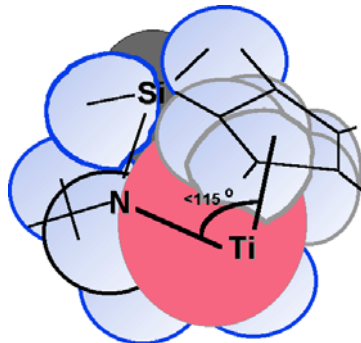
Constrained Geometry Catalyst (Ref. Dow Chemical Company)
